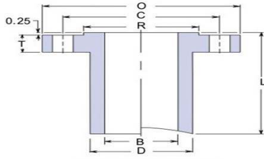
LONG WELD NECK "LWN"
